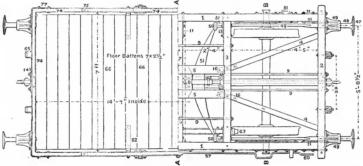
Fig. 349. Plan of Floor and Underframe.
